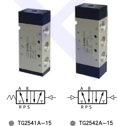
● TG2541A-15 ● TG2542A-15
