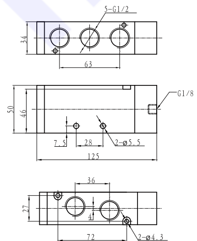
● TG2541A-15 ● TG2542A-15
