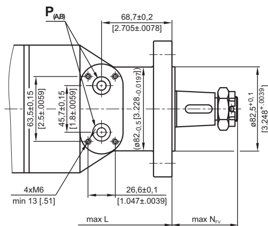
HWFV Wheel mount, six holes, relief valves
