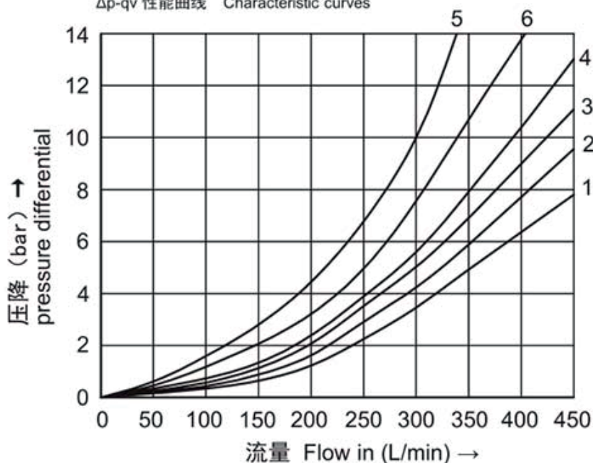
Δp-qv 性能曲线 Characteristic curves
